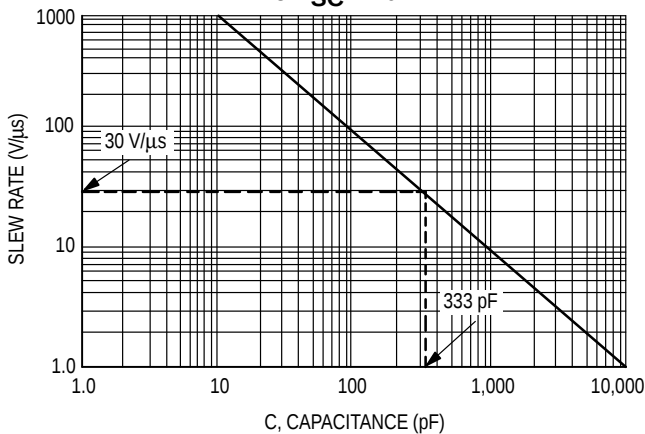
Figure 12. Slew Rate versus Capacitance for I_{OS} = 10 mA
