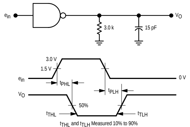
Figure 6. Switching Response
